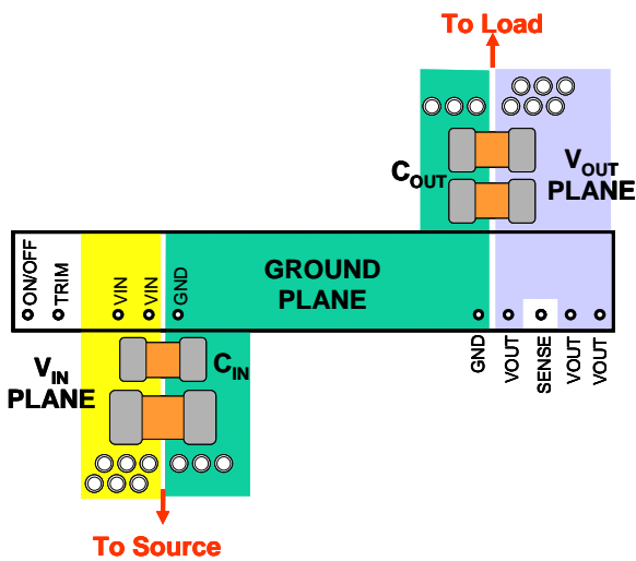
Fig. 5. Simplified layout for the Austin Lynx and SuperLynx series SIP modules.
