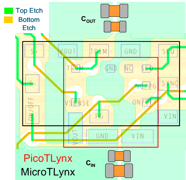
Fig. 7. Dual layout for the PicoTLynx and MicroTLynx modules.
